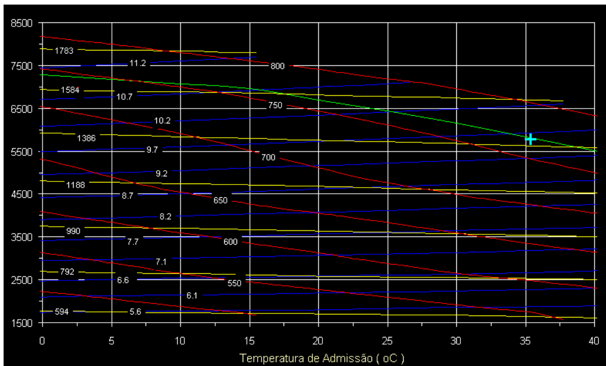
Figura 16 – Curva de Performance Turbinas Taurus 60
